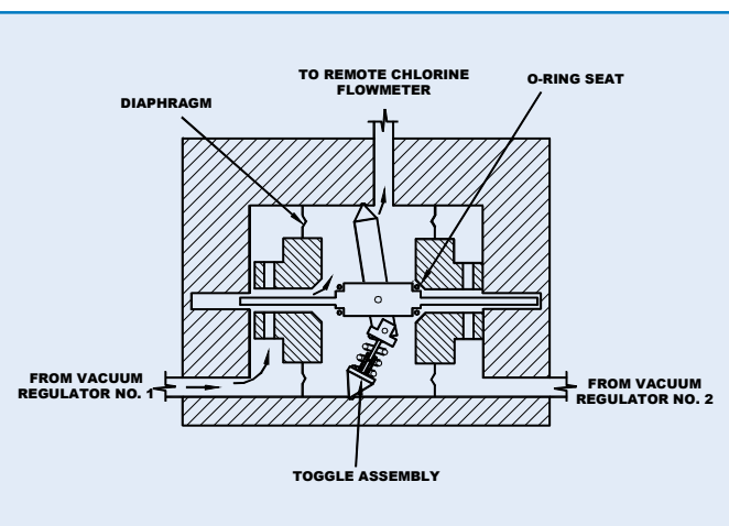
Figure 2 - Automatic Switchover Flow Diagram
