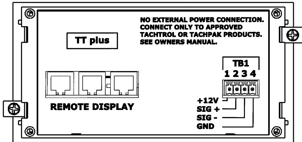
REAR VIEW - CONNECTIONS
