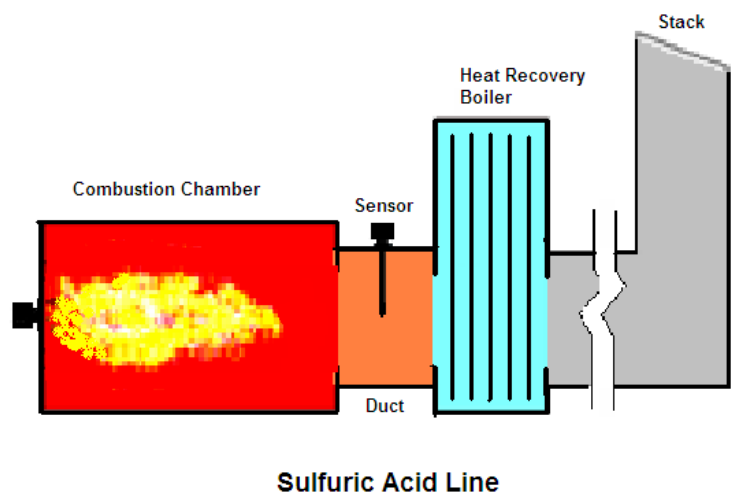
Figure 1. Typical installation location for a high-temp oxygen analyzer in the sulphuric acid production process.
